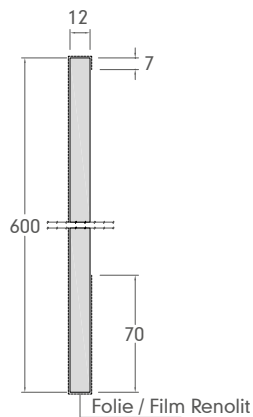
RLK 600 (3660 mm)
