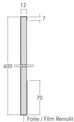
RLK 600 (3660 mm)
